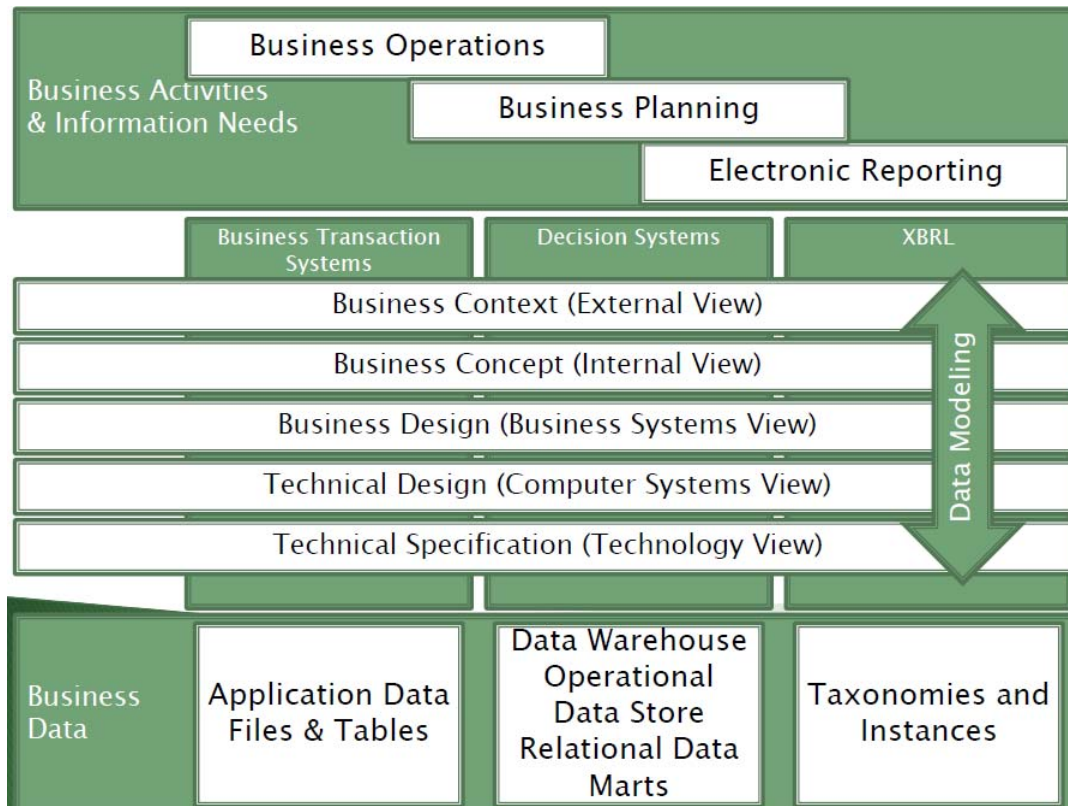
Figure 1 — The Business Overview to Rollout XBRL reporting
