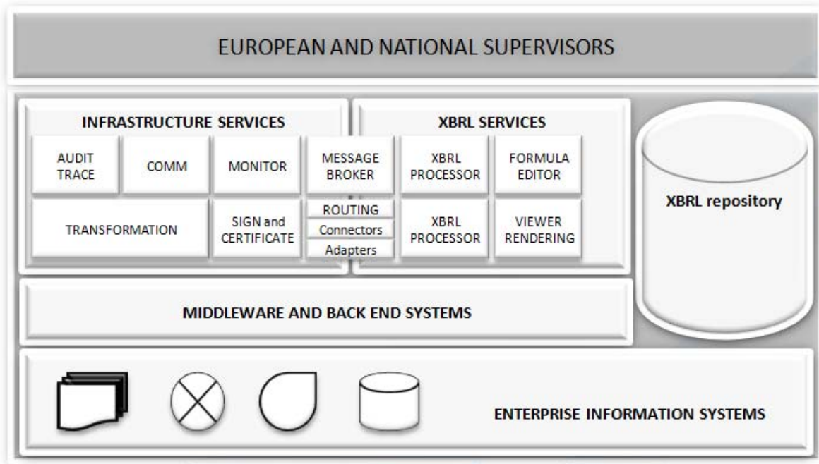
Figure 7 — XBRL Technical Architecture of Reference Overview
