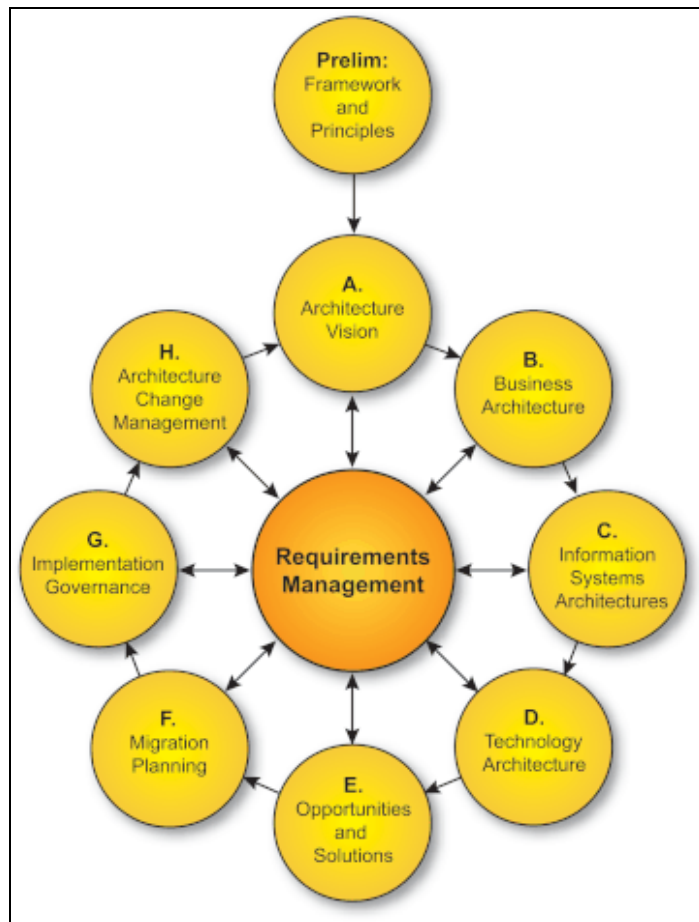
Figure 6 — TOGAF Architecture Lifecycle diagram
